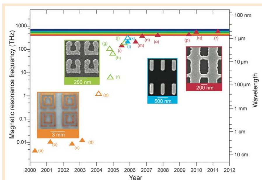
Figure 7. Fabrication progress of negative index materials vs year. This figure is taken from the article in Nature Photonics 5, 523 (2011) written by Soukoulis and Wegener [4].
