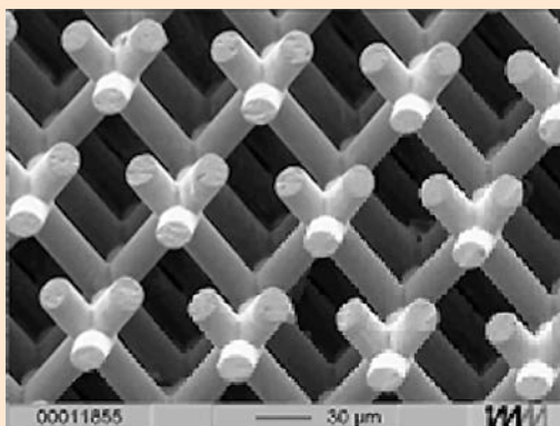
Figure 5. The “three-cylinder” photonic crystal made from negative tone resist [1].
