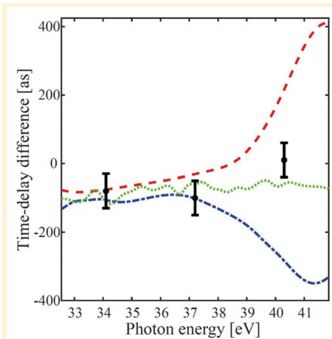
Figure 3. Measured relative ionization time delay between the 3s and 3p sub-shells in argon in comparison with different calculation methods. The figure is adapted from [18] with additional calculations from [19].
