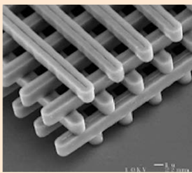
Figure 4. Electron-microscope image of a “woodpile” photonic crystal made by silicon with a complete band gap at 12 \mu\text{m} [1].
